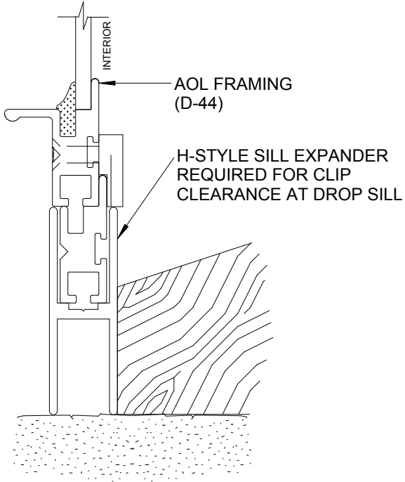
3 SILL DETAIL SCALE: FULL
