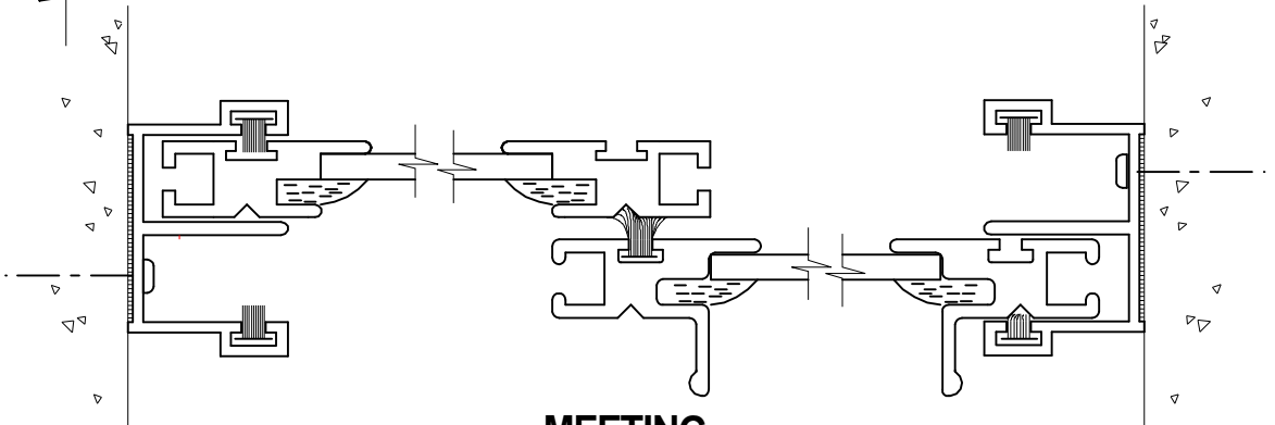
4 MEETING RAIL DETAIL SCALE: FULL
