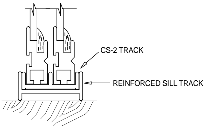
3 REINFORCED SILL DETAIL SCALE: FULL Optional
