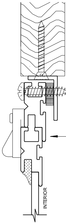
1 HEAD DETAIL SCALE: FULL
