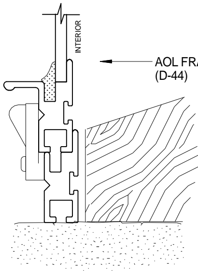
3 SILL DETAIL SCALE: FULL
